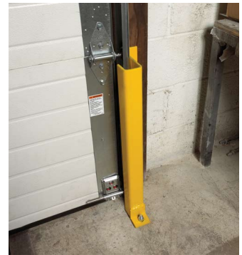
Over Head Door Protector
